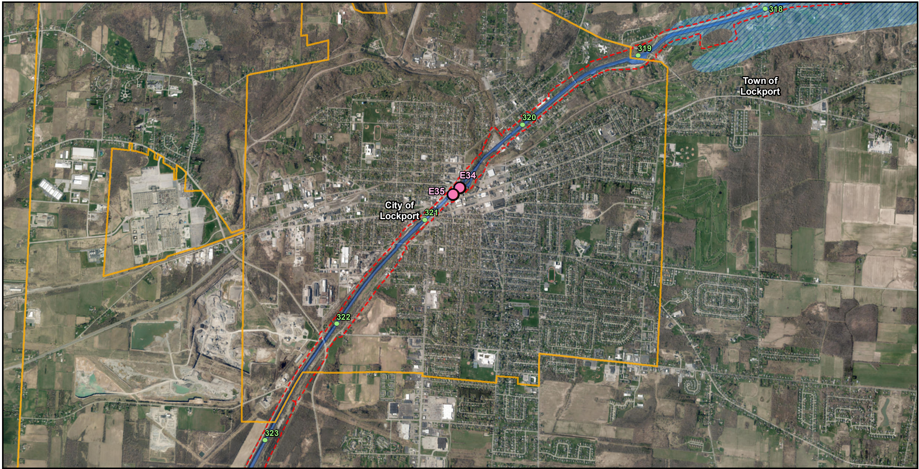
Figure 116F: Aquifers
